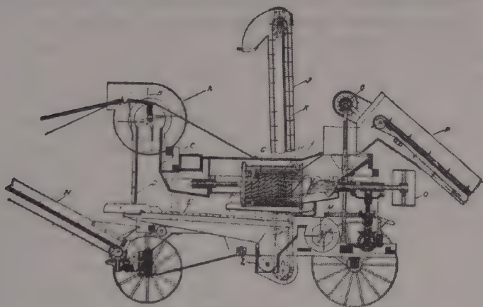
Fig. 191. A section of a cylinder sheller.
