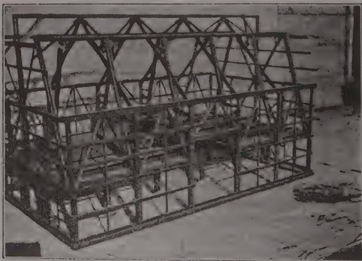
Fig. 288. A model Shawver barn frame.
