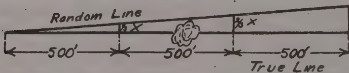
Fig. 8. Sketch showing method of locating points on a desired line between two points not visible from each other from a random line.
