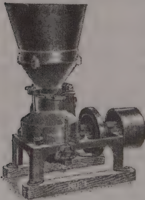
Fig. 187. A belt-driven feed mill.
