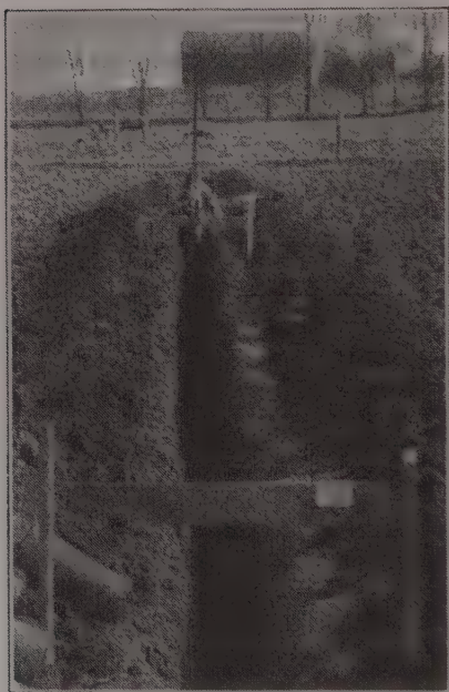
Fig. 57. The target method of grading tile ditches.
