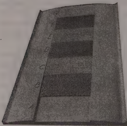
Fig. 36. Model of a bituminous macadam road made by the penetration method. A represents the prepared sub-grade. B represents the first course of stone, and C the second course. D shows the first application of bitumen. E shows the application of a course of stone chips. F shows second application of bitumen. G shows the completed road with a layer of clean stone chips, lightly rolled. (Bul. 36, Office of Public Roads, U. S. Dept. of Agr.)
