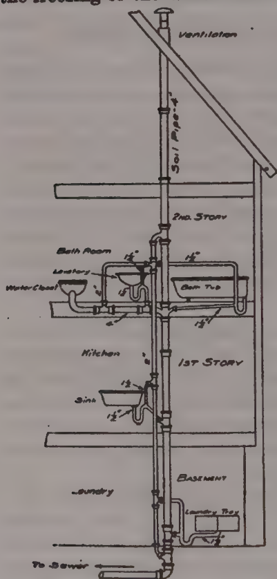
Fig. 207. A plumbing system for a two-story house. The vent pipe may be omitted with safety in country residences. (Mo. Eng. Exp. Sta. Bul.)
