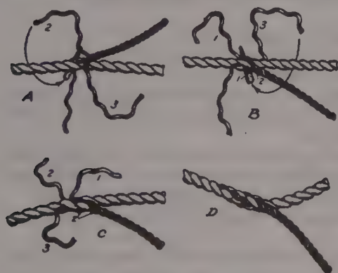
Fig. 341. Side splice.
