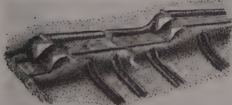
Fig. 76. Manner of placing tubes in ditch bank for furrow irrigation. (Farmer's Bul. 373, U. S. Dept. of Agr.)
