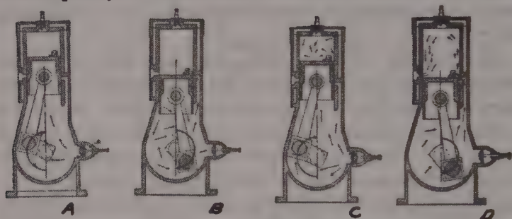
Fig. 222. Illustrating the operations which take place in the two-stroke cycle engine. A, suction into crank case. B, compression in crank case. C, compression in cylinder combined with A. D, expansion in cylinder combined with B. (From Farm Machinery and Farm Motors.)
