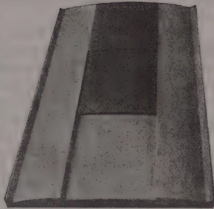
Fig. 83. Model of a gravel road illustrating the trench method of construction. A shows prepared sub-grade; B, first course of gravel; C, upper course of gravel. (Bul. 36, Office of Public Roads, U. S. Dept. of Agr.)
