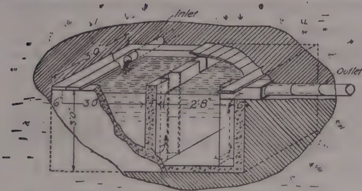
Fig. 808. A general view of a septic tank arranged to be connected with an underground irrigation or filter system without a siphon. (After Stewart.)
