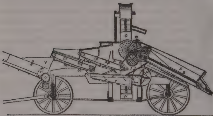
Fig. 190. A section of a picker-wheel sheller.
