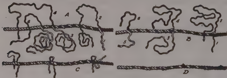
Fig. 340. Long splice, three-strand rope.
