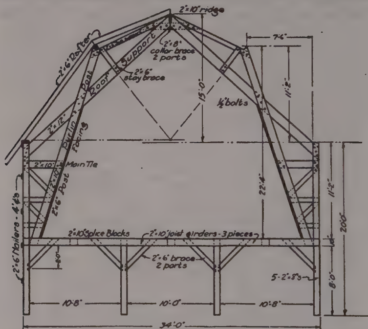
Fig. 290. A sketch of the Shawver barn frame.
