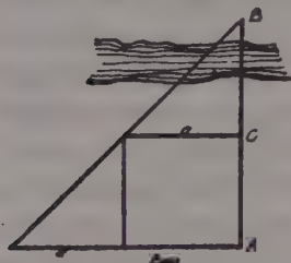
Fig. 9. Sketch showing method of measuring to an inaccessible point.
