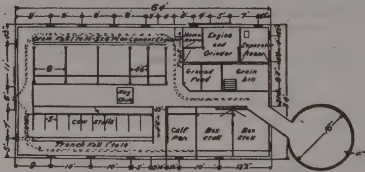
Fig. 284. Floor plan of a general farm barn.
