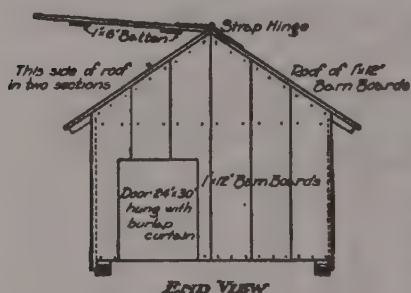
Fig. 266. End elevation of gable-roof colony hog house.
