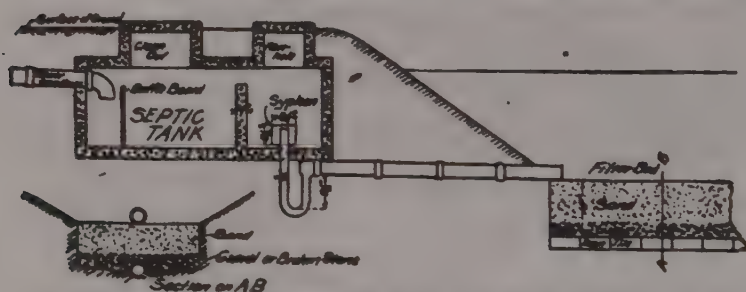
Fig. 209. Section of a septic tank made entirely of concrete. It has a siphon and a filter bed of sand and gravel.
