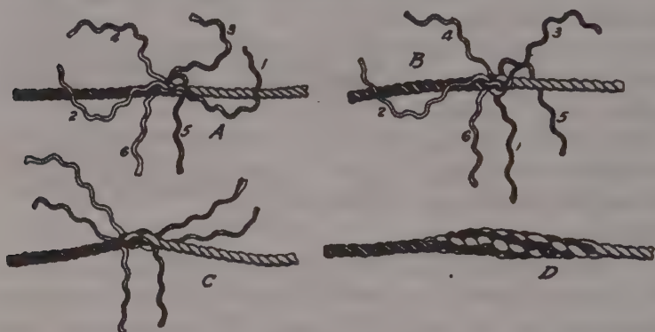
Fig. 339. Short splice.
