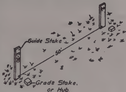
Fig. 49. Grade stakes, or hubs, and guide stakes.
