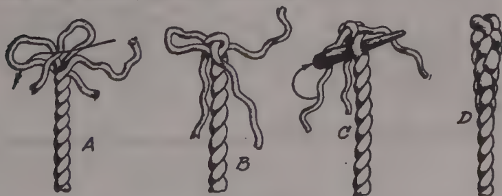
Fig. 338. Crowning.
