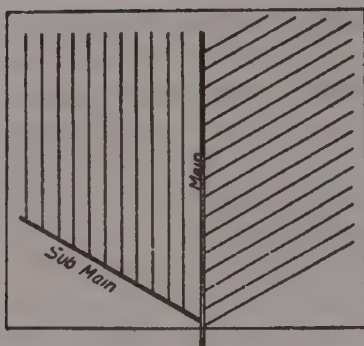
Gridiron System
