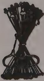
Fig. 1. The Gunter's chain, folded.
