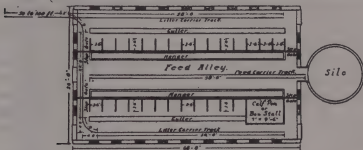
Fig. 281. Floor plan of a modern dairy barn.
