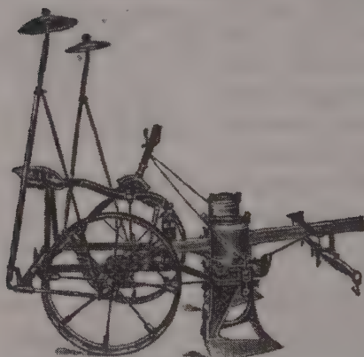
Fig. 144. A corn planter with stub shoe furrow-openers.
