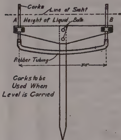
Fig. 31. A home made water level.
