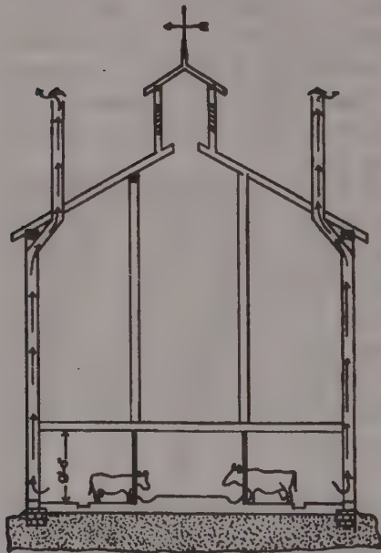
Fig. 322. Showing one method of arranging the outlet flues in the King system. The flues may be brought together to form a common outlet.
