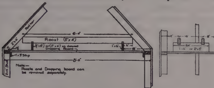
Fig. 274. Detail of roosts and dropping board.
