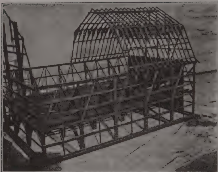
Fig. 287. A model Wing joist barn frame.
