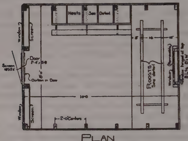
Fig. 271. Plan of an A-shaped colony poultry house. (La. Exp. Sta., Bul. 122.)
