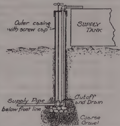
Fig. 306. A satisfactory method of installing exposed hydrants.
