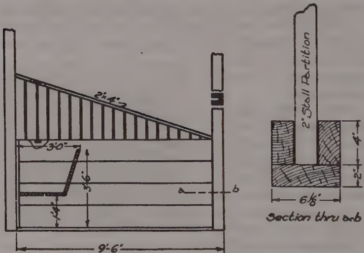
Fig. 286. Detail of construction of a horse stall.
