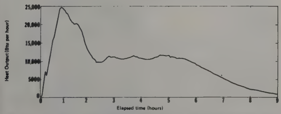
Figure 7-7. The heat output of a Morss 28 stove during a particular run involving one full loading with fuel at the beginning and no subsequent adjustments. The surge at the beginning is typical when non-automatic stoves are operated at medium power, and probably corresponds to the burning of combustible gases, which are most abundant in the early portions of a fire. 2
