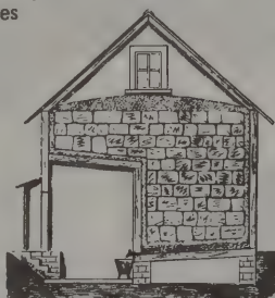
FIG. 140.—ICE HOUSE AND REFRIGERATOR.
